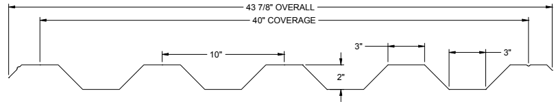
ALUMINUM PANEL
