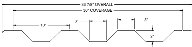
STEEL PANEL
